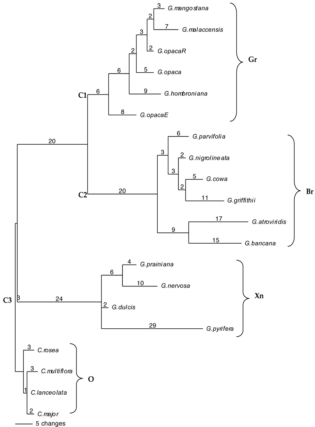
Fig. 3: One of the most parsimonious trees based on the accD-psaL sequence data from 14 species of Garcinia. Figures are tree length based on the numbers of DNA substitution changes. Key: O-Clusia outgroup Xn-Section Xanthochymus Gr-Section Garcinia Br-Section Brindonia
